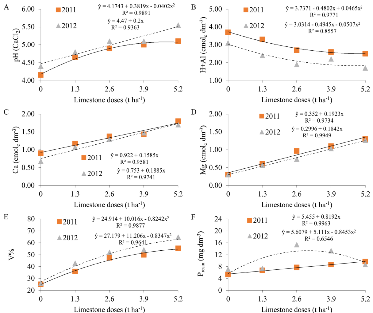
Figure 2. Regression models fitted to the data of the variables pH (A), potential acidity (H+Al - B), Ca (C), Mg content (D), base saturation (V% - E) and P (F) content of the soil submitted to limestone doses, in two years of cultivation (2011 and 2012), in Teresina-PI
