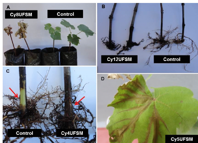
Figure 1. Symptoms of black foot disease in Vitis labrusca cv. Bordô: A) drying of shoots after inoculation with Cy8UFMSM versus control; B) root mass reduction after inoculation with Cy12UFMSM versus control; C) crown necrosis after inoculation with Cy4UFMSM versus control; D) necrosis of the leaf ribs after inoculation with Cy5UFMSM
